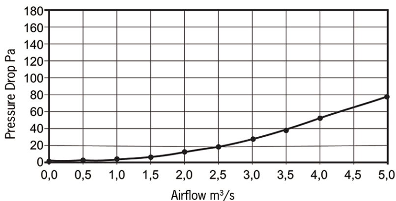
Pressure Drop
